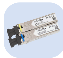
1.25G SFP MODULE KIT, SINGLE-MODE 20KM (S- 3553LC20D)
