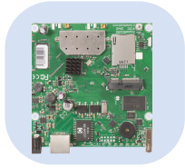
WIRELESS ROUTERBOARD (RB912UAG- 2HPND)
